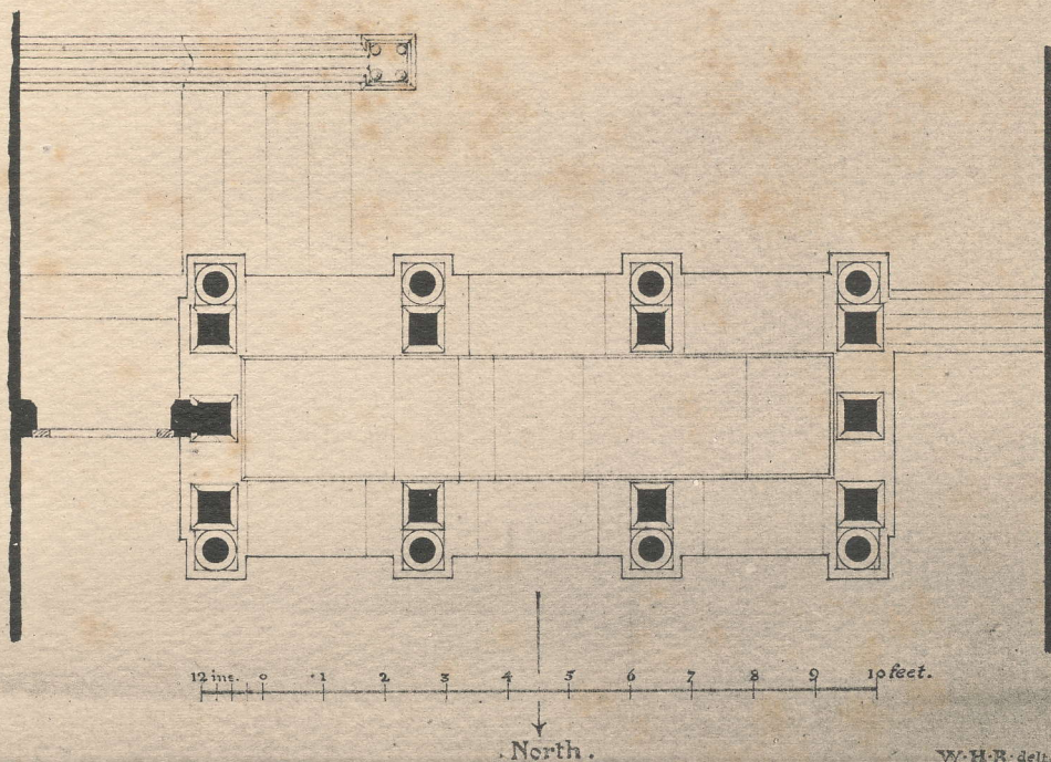
Fig. 3. Plan of the Monument.
